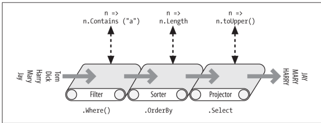
Figure 6. Chaining query operators
