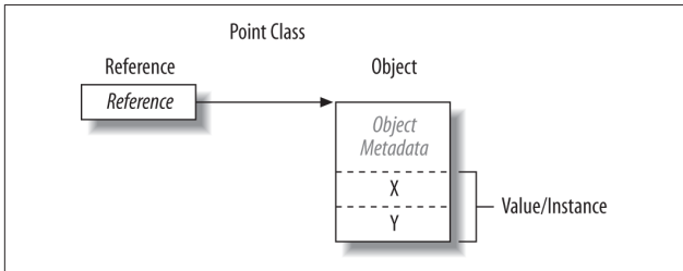
Figure 3. A reference-type instance in memory
