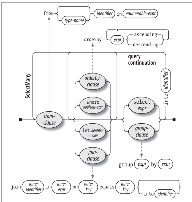
Figure 7. Query expression syntax
