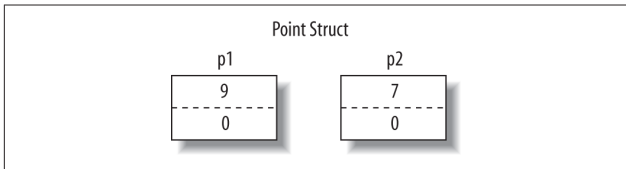
Figure 2. Assignment copies a value-type instance
