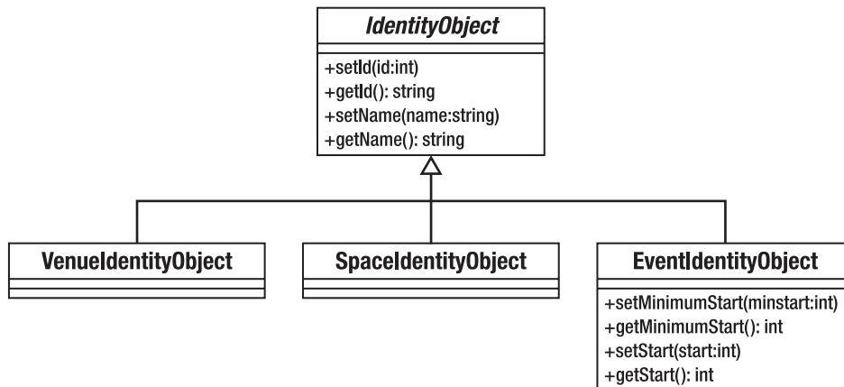
Figure 13–9. Managing query criteria with identity objects
