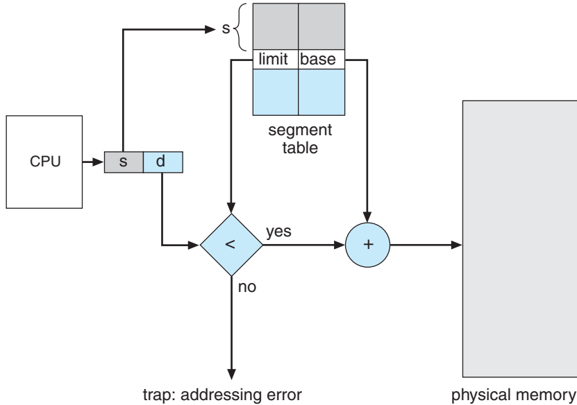
Figure 8.8 Segmentation hardware.
