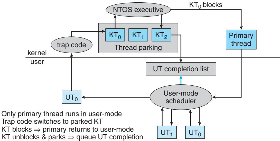
Figure 19.11 User-mode scheduling.
