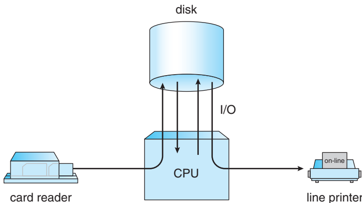
Figure 20.5 Spooling.
