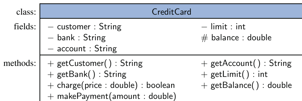
Figure 1.5: A UML Class diagram for the CreditCard class from Section 1.7.
