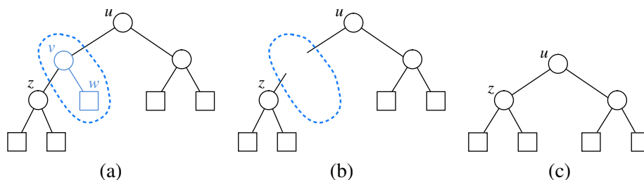
Figure 8.8: Operation that removes an external node and its parent node, used in the justification of Proposition 8.8.
