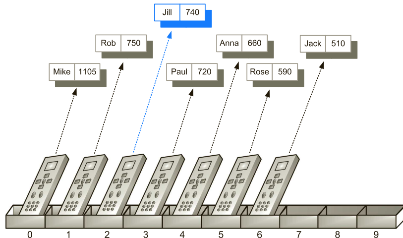
Figure 3.3: Adding a reference to Jill’s GameEntry object to the board array. The reference can now be inserted at index 2, since we have shifted all references to GameEntry objects with scores less than the new one to the right.
