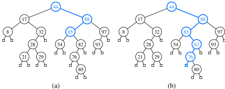
Figure 11.2: (a) A successful search for key 65 in a binary search tree; (b) an unsuccessful search for key 68 that terminates at the leaf to the left of the key 76.
