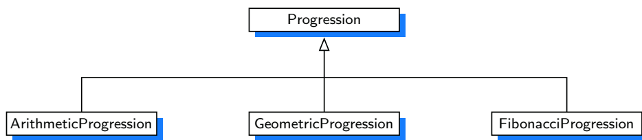
Figure 2.5: An overview of our hierarchy of progression classes.
