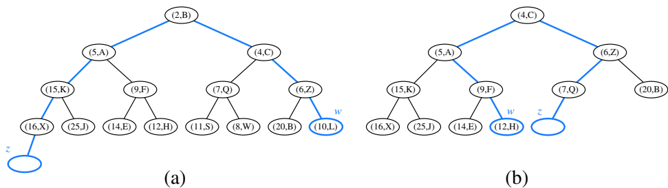
Figure 9.12: Two cases of updating the last node in a complete binary tree after operation insert or remove . Node w is the last node before operation insert or after operation remove . Node z is the last node after operation insert or before operation remove .
