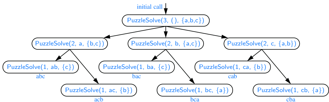
Figure 5.14: Recursion trace for an execution of \text{PuzzleSolve}(3, S, U) , where S is empty and U = \{a, b, c\} . This execution generates and tests all permutations of a , b , and c . We show the permutations generated directly below their respective boxes.
