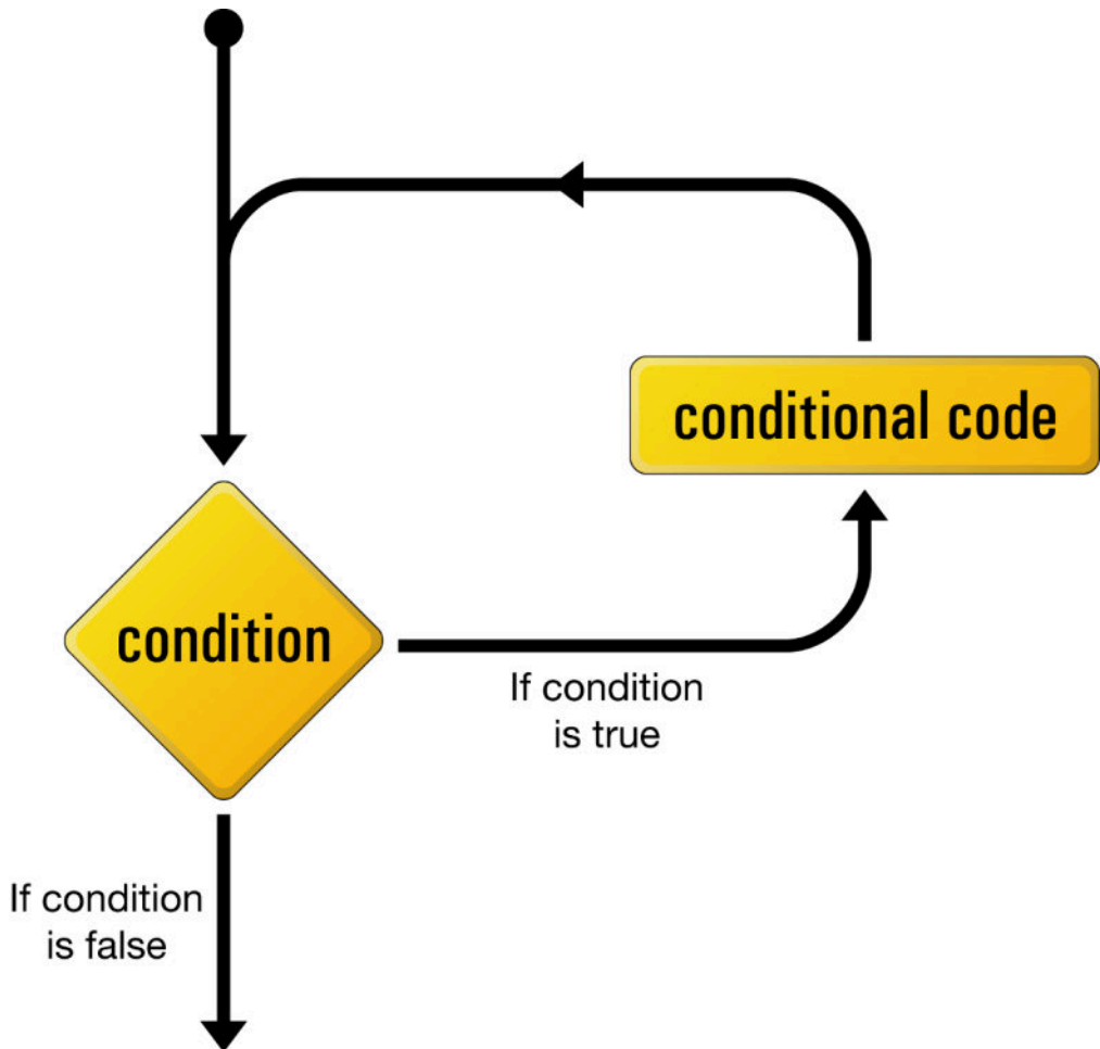
2-13. The logical flow of a while loop
