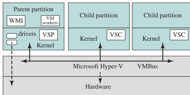
Figure 14.9 Hyper-V
