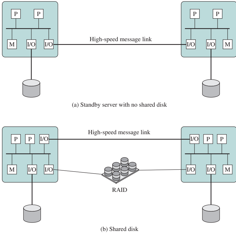
Figure 16.13 Cluster Configurations
