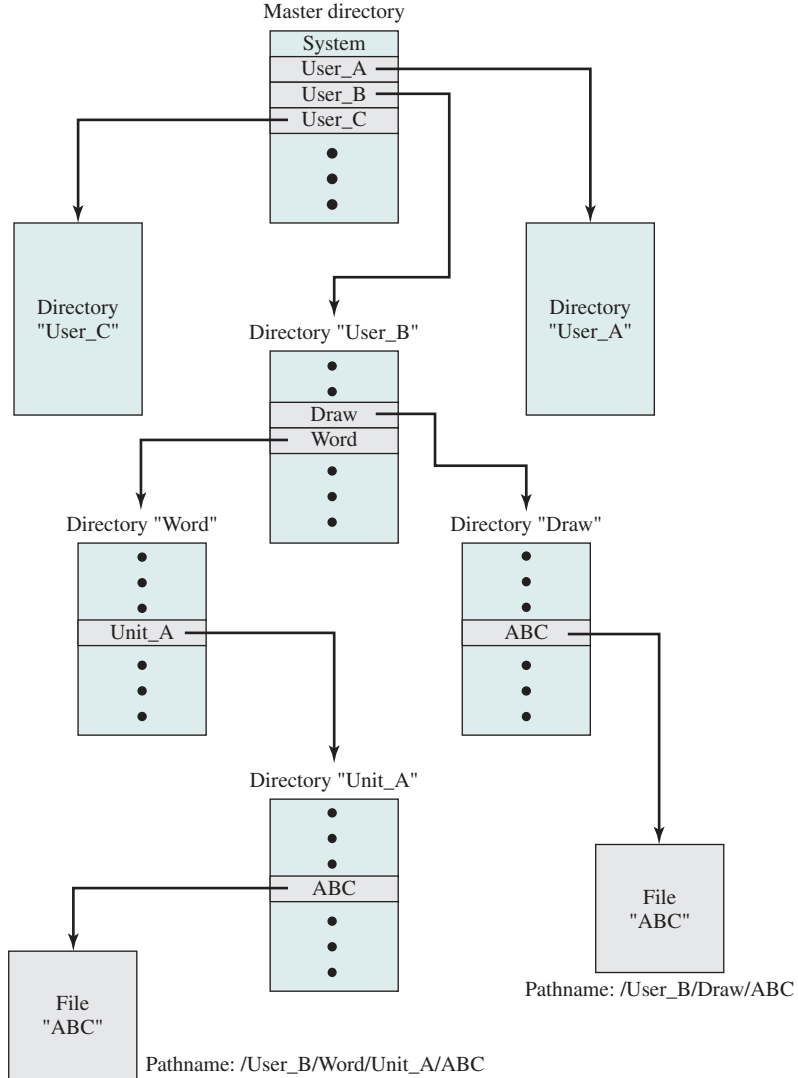
Figure 12.7 Example of Tree-Structured Directory
