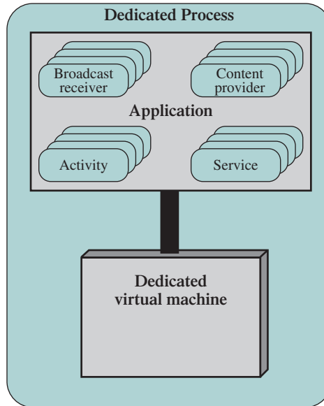
Figure 4.16 Android Application
