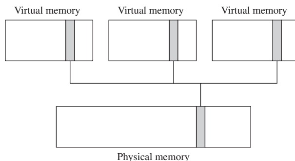
Figure 14.4 Page Sharing
