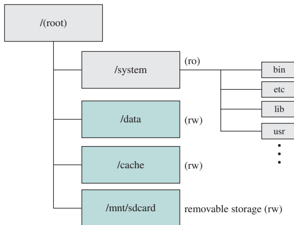
Figure 12.21 Typical Directory Tree of Android
