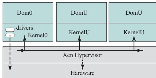
Figure 14.8 Xen
