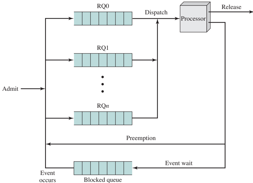
Figure 9.4 Priority Queueing
