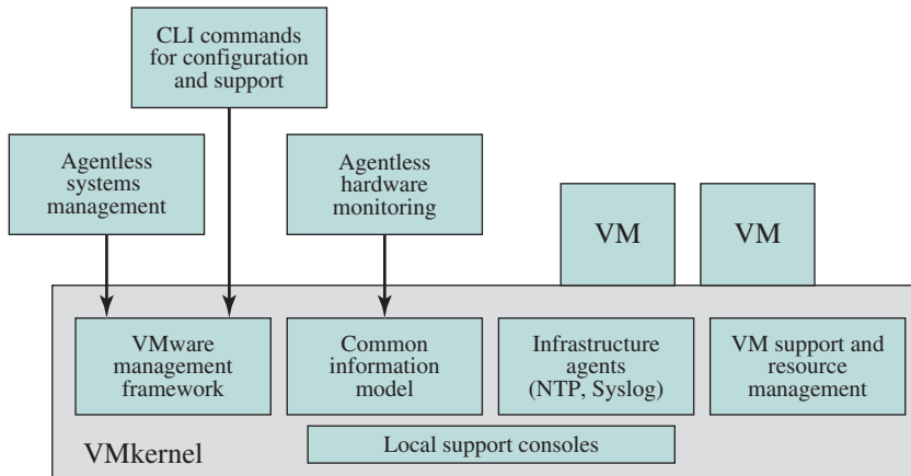
Figure 14.7 ESXi
