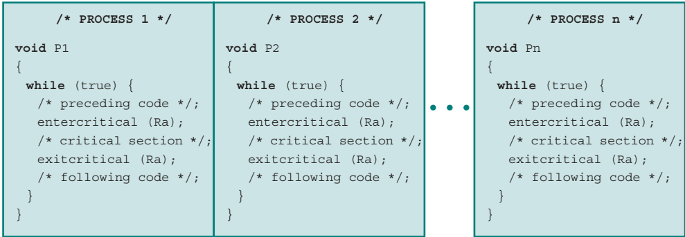
Figure 5.1 Illustration of Mutual Exclusion
