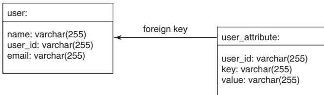
Figure 2.18 Generic data model
