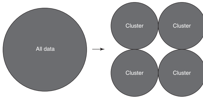
Figure 7.7 Clustering data
