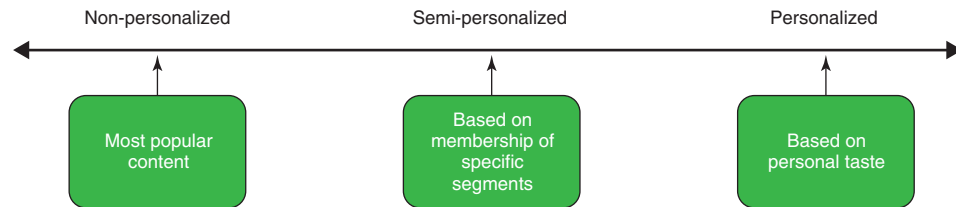
Figure 1.11 Personalization levels
