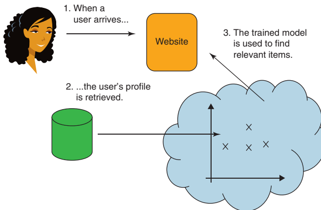
Figure 10.5 The item retriever returning recommendations with content-based filtering online.
