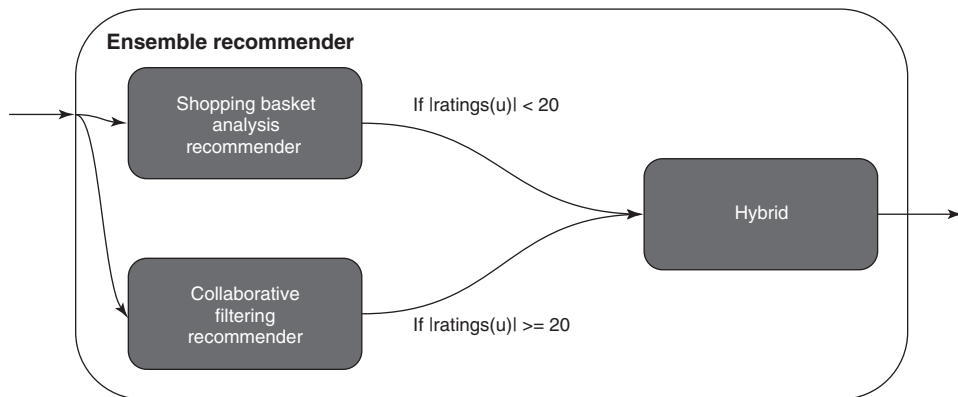
Figure 12.8 An example of a switching ensemble where users with more than 20 ratings receive output from one recommender, while users with fewer than 20 receive recommendations from another.
