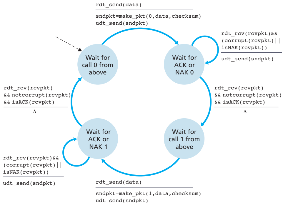
Figure 3.11 ♦ rdt2.1 sender
