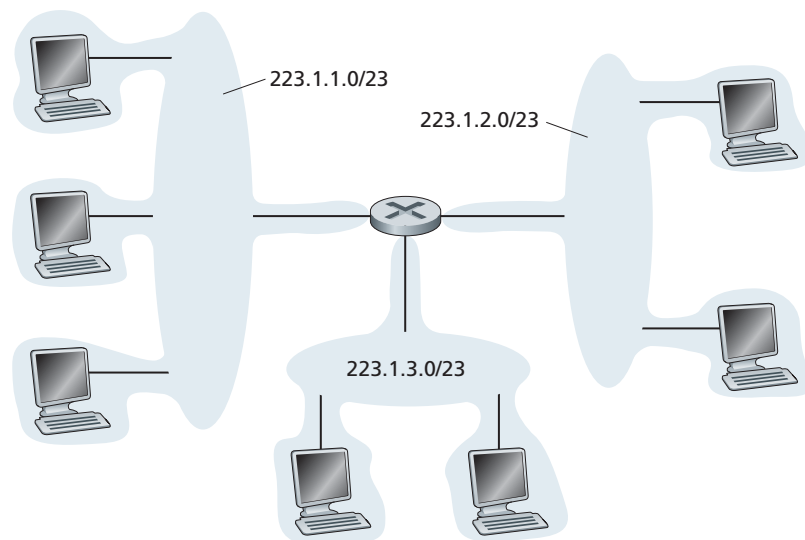
Figure 4.16 ♦ Subnet addresses
