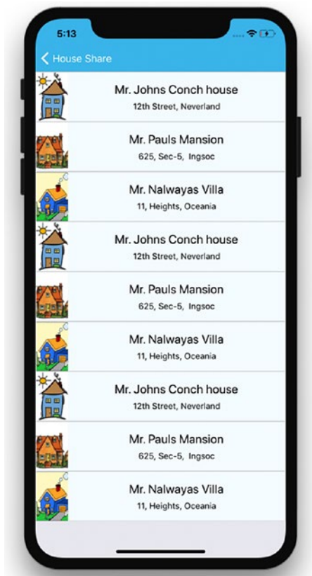
Figure 4-15. Scrollable addresses
