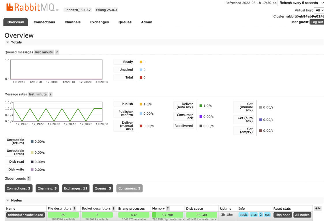
Figure 8.20: The RabbitMQ management dashboard displaying connections and queues
