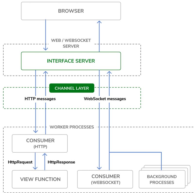
Figure 16.3: The Django Channels request/response cycle
