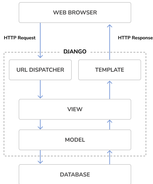
Figure 1.1: The Django architecture
