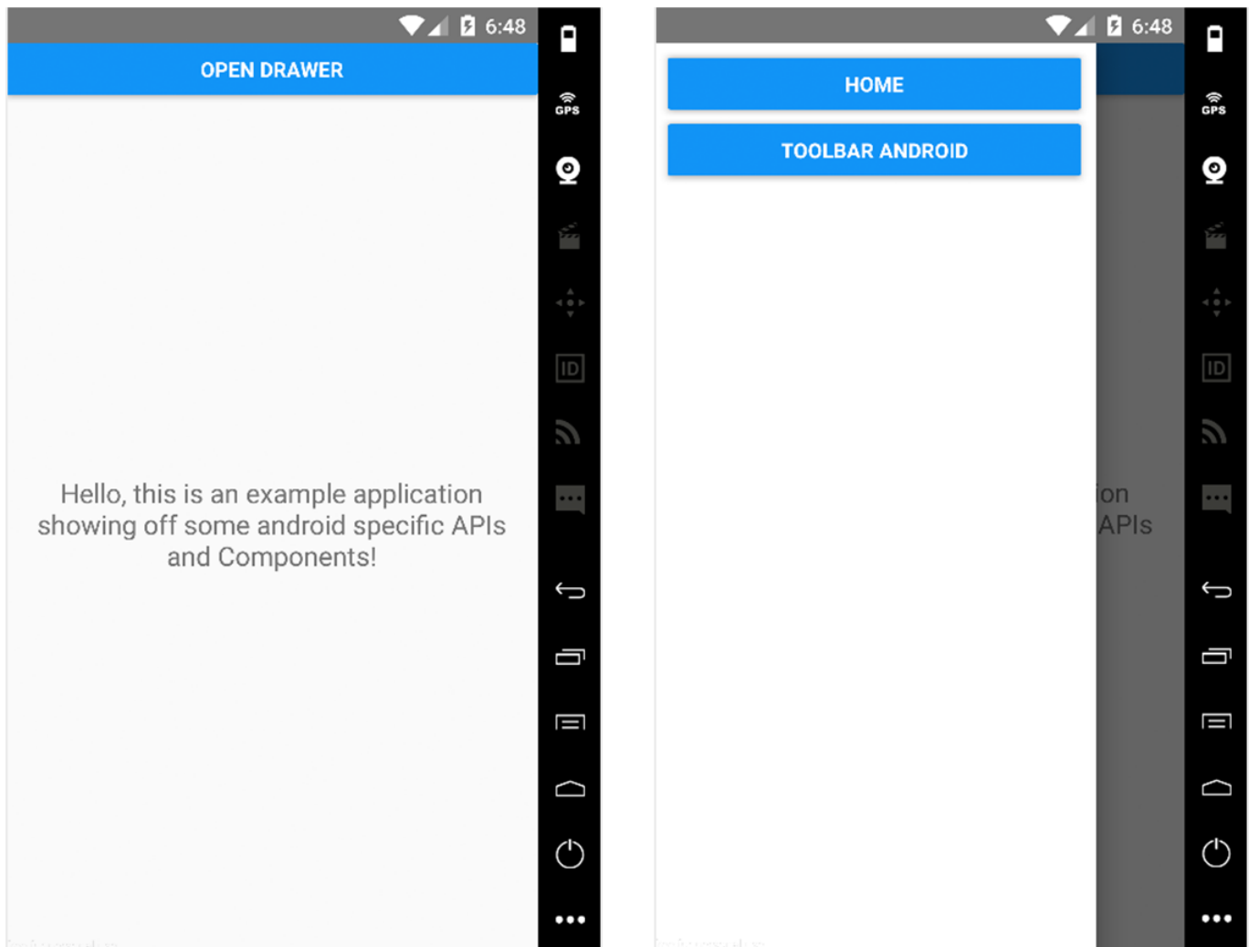
Figure 11.1 Initial layout of the application using DrawerLayoutAndroid . The button at the top in the first screen, Open Drawer, will call a method that opens the drawer. The second screen is the opened drawer.
