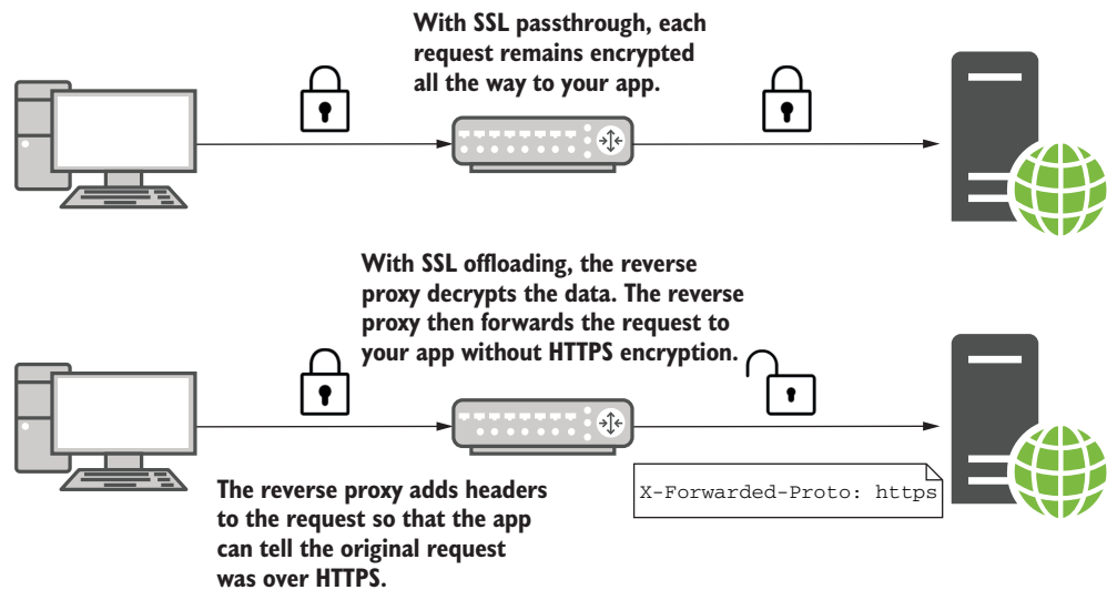
Figure 18.2 You have two options when adding HTTPS to an ASP.NET Core app: SSL passthrough and SSL offloading. In SSL passthrough, the data is encrypted all the way to your ASP.NET Core app. For SSL termination, the reverse proxy handles decrypting the data, so your app doesn't have to.
