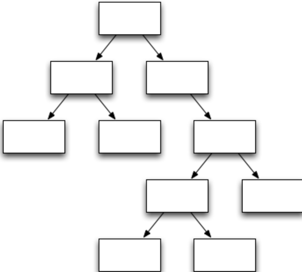
Component tree
