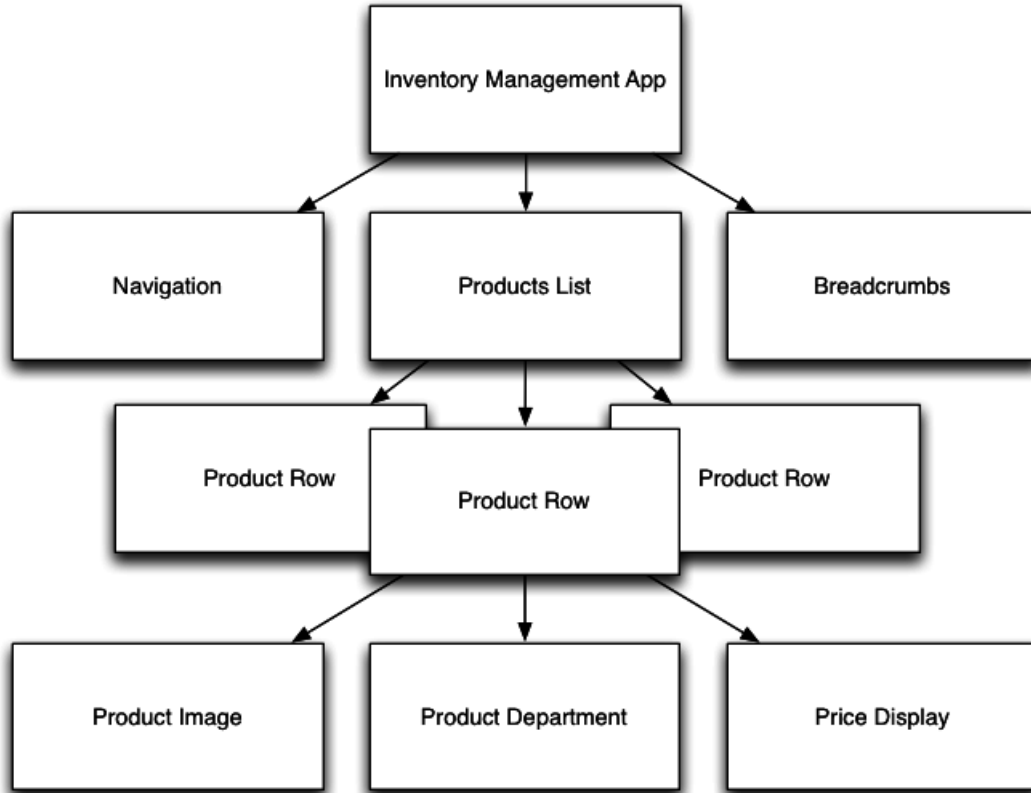
App Tree Diagram
