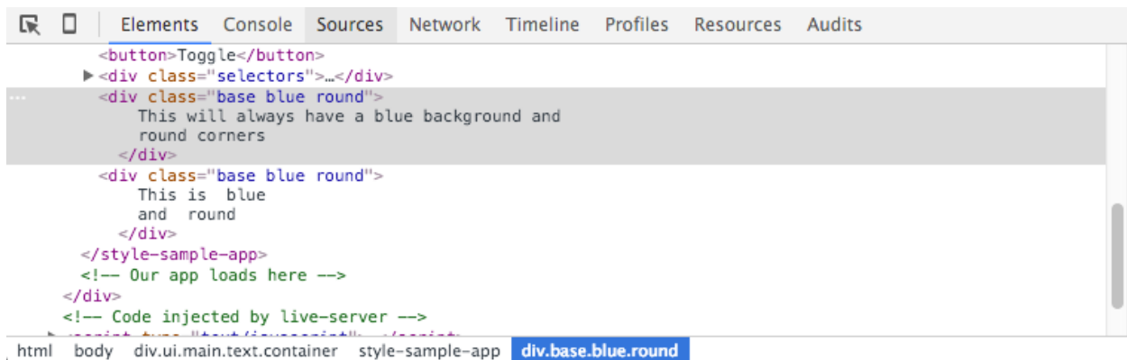
Classes from both the attribute and directive
