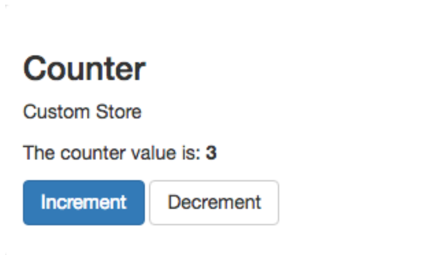
Counter App
